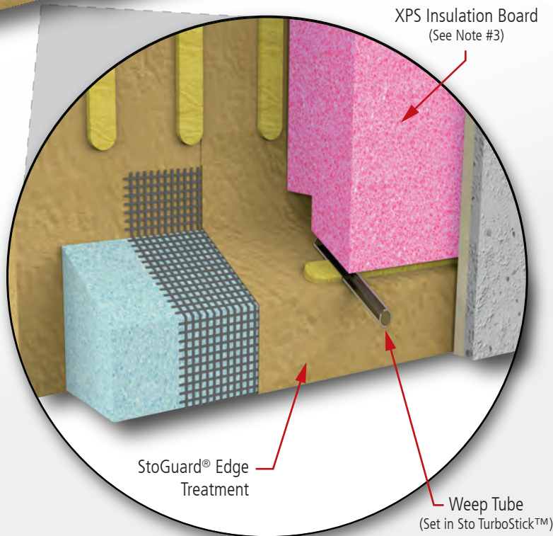
Sto Wedge Patented integral drainage at bottom of panel
